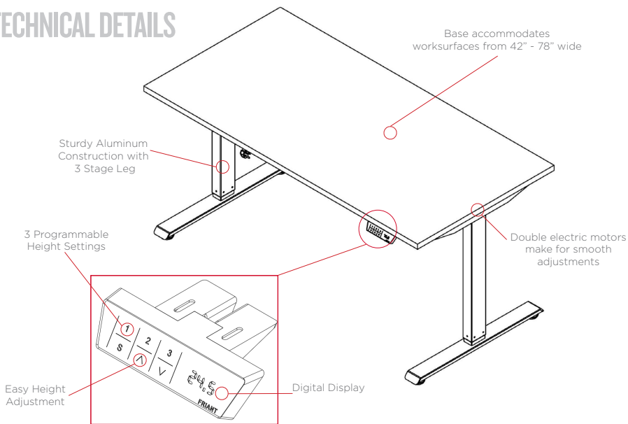
Digital display with three programmable presets
